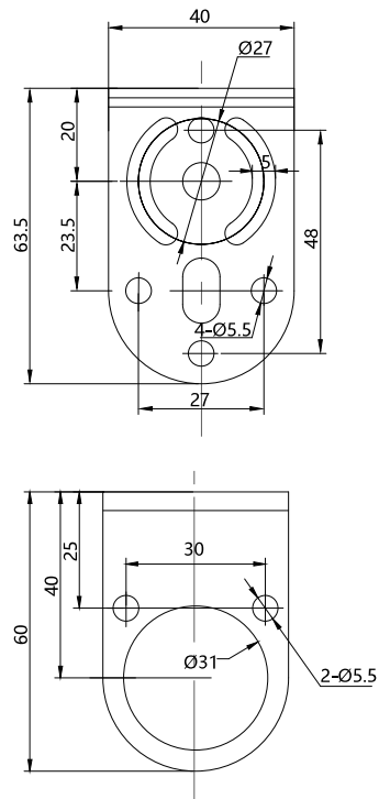
XS-C100 L-Bracket
