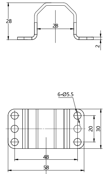
XS-C110 D28 Lock the bracket
