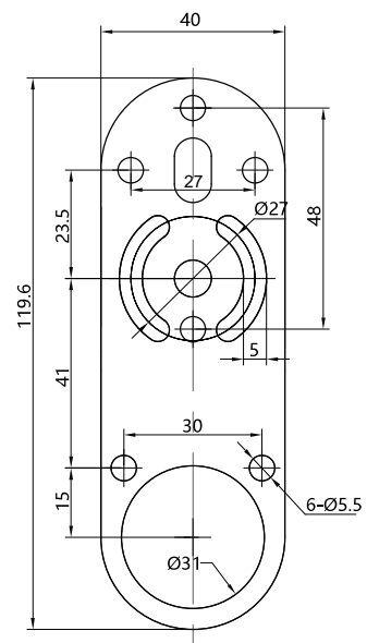
XS-C101 Horizontal Bracket
