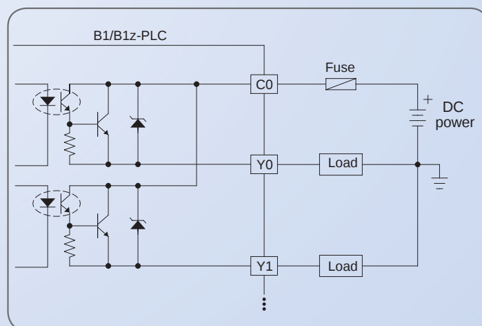
Wiring of transistor single-end SOURCE output
