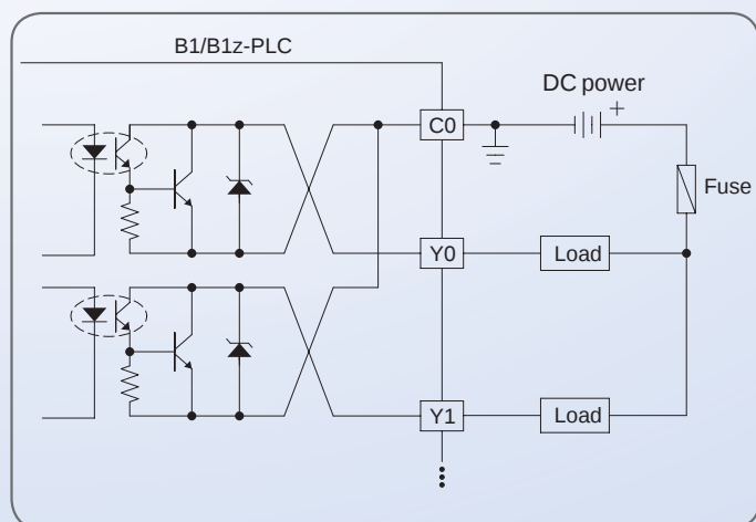
Wiring of transistor single-end SINK output
