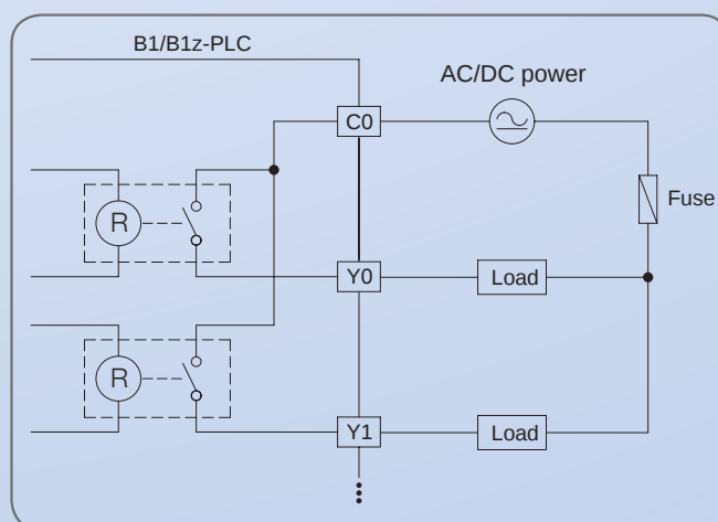
Wiring of relay single-end output
